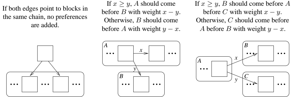
Figure 8: Adding branch prediction preferences for architectures that predict backward conditional branches taken and forward conditional branches not taken.
