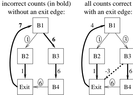
Figure 4: Trace and control-flow graphs illustrating re-entry into fact with and without an exit edge.
