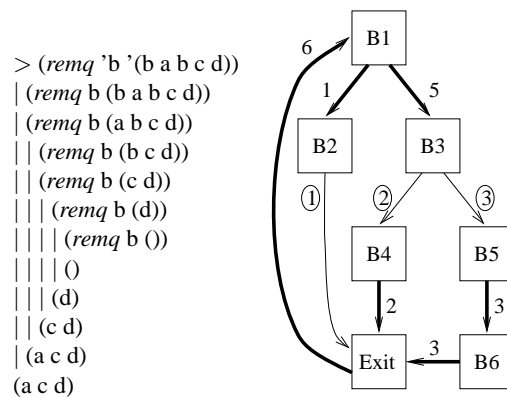
Figure 1: remq source, basic blocks, sample trace, and control-flow graph with thick, uninstrumented edges from one of the twelve maximal spanning trees and encircled counts for the remaining, instrumented edges.
