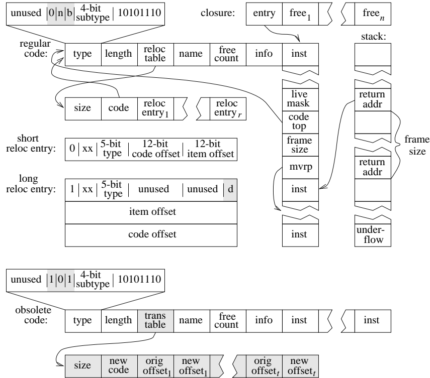
Figure 7: Representation of closures, code objects, and stacks with the infrastructure for dynamic recompilation highlighted.
