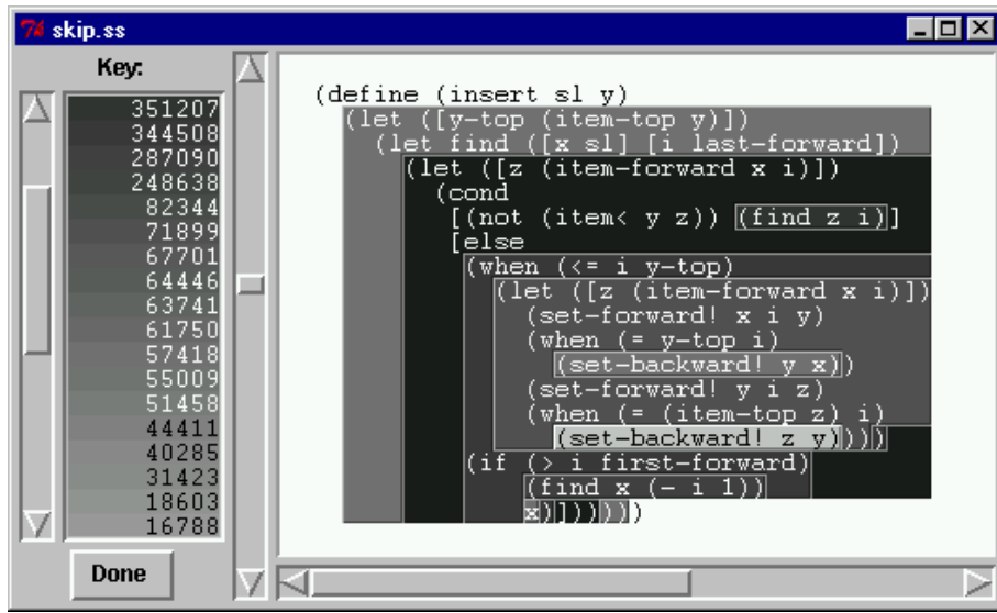
Figure 6: A section of code displayed using darker shades for more frequently executed code and lighter shades for less frequently executed code.
