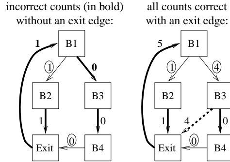
Figure 3: Trace and control-flow graphs illustrating nonlocal exit from fact with and without an exit edge.
